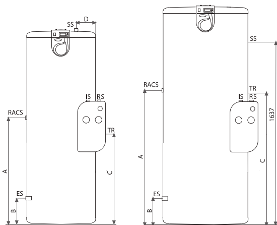
DS-PACK 190-300-500
